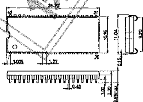
SANYO: SOJ40
