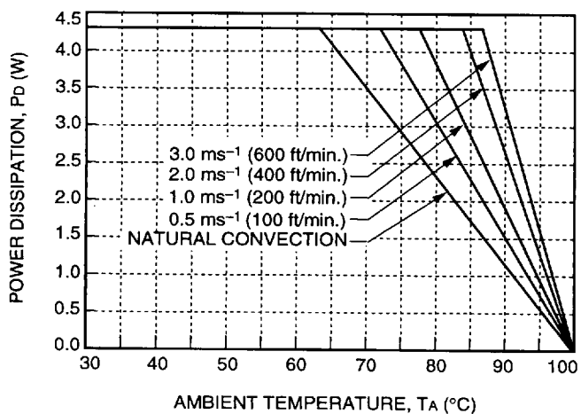
Figure 12. Forced Convection Power Derating with No Heat Sink; Either Orientation
