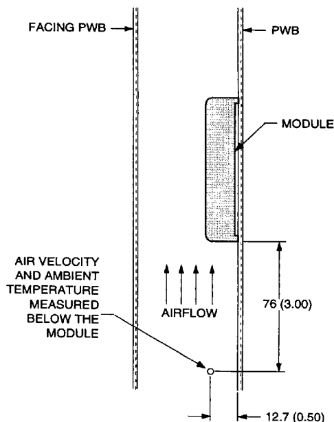
Figure 14. Experimental Test Setup
