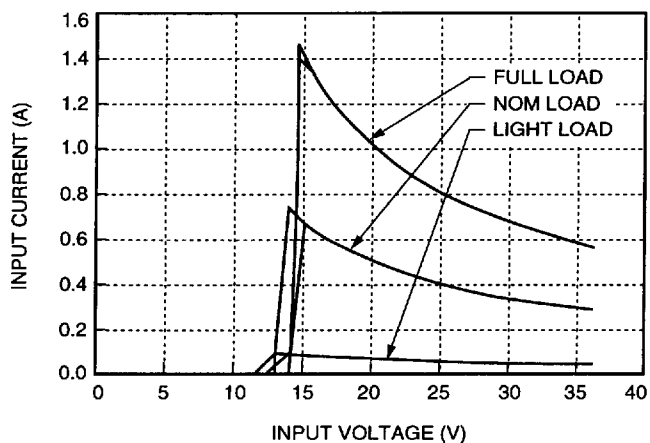
Figure 1. LC016AJ Typical Input Characteristics, T_A = 25^\circ\text{C}
