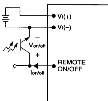
Figure 10. Remote On/Off Implementation
