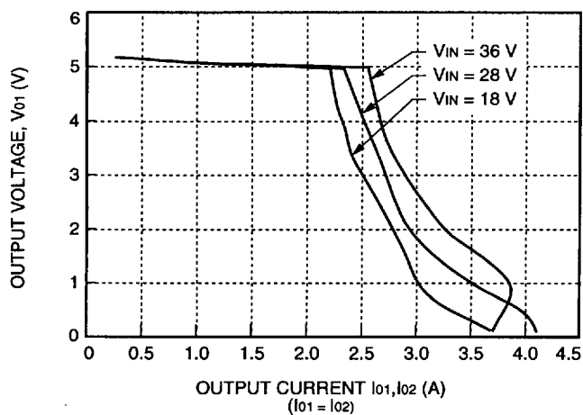
Figure 2. LC016AJ Typical Output Characteristics, T_A = 25^\circ\text{C}
