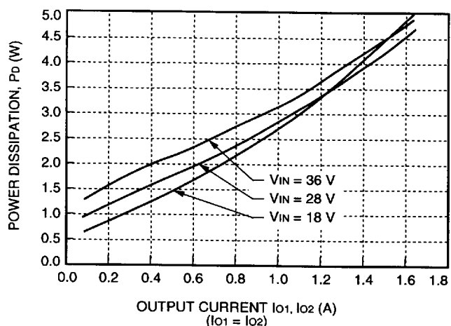
Figure 13. LC016AJ Power Dissipation vs. Output Current, T_A = 25^\circ\text{C}
