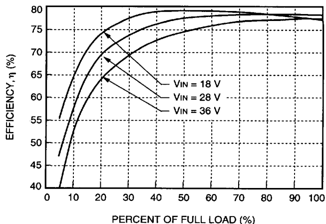
Figure 3. LC016AJ Typical Converter Efficiency vs. Output Current, T_A = 25^\circ\text{C}
