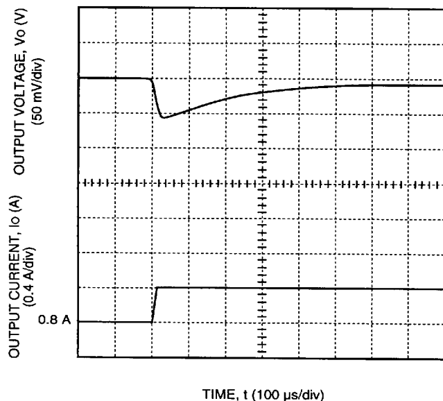
Figure 5. LC016AJ Typical Output Voltage for a Step Load Change from 50% to 75%
