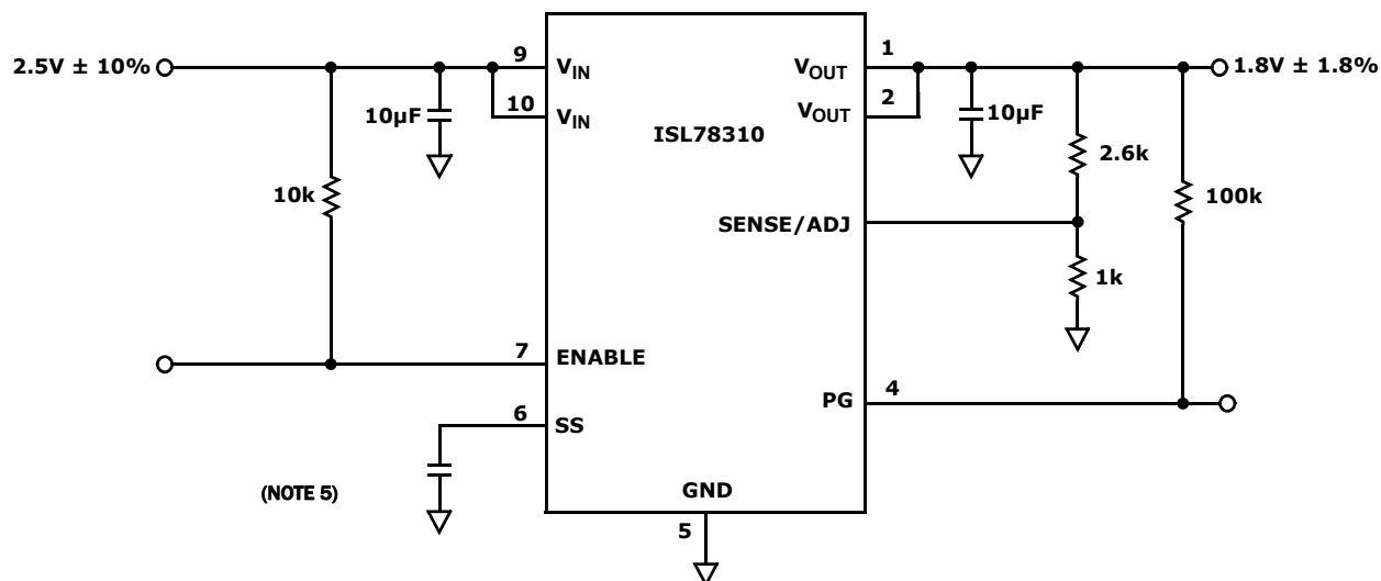
FIGURE 2. ADJUSTABLE TYPICAL APPLICATION DIAGRAM
