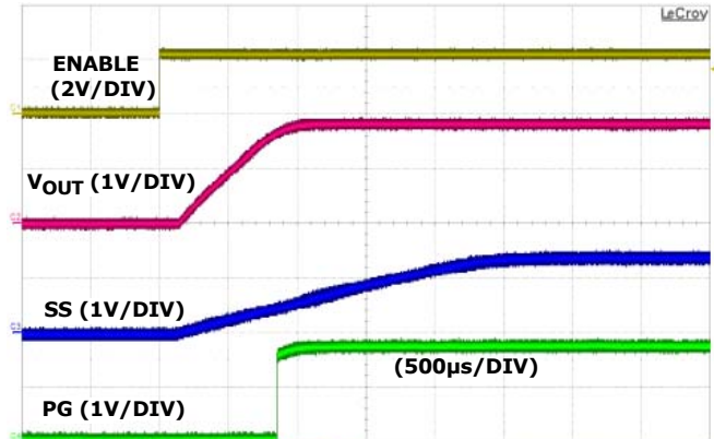
FIGURE 10. ENABLE START-UP
