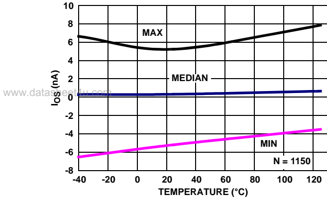
FIGURE 30. I_{OS} vs TEMPERATURE, V_+, V_- = \pm 2.5V
