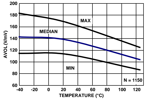
FIGURE 35. AVOL vs TEMPERATURE, V_+, V_- = \pm 2.5V, V_O = -2V \text{ TO } +2V, R_L = 1k
