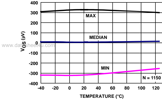
FIGURE 24. V_{OS} vs TEMPERATURE, V_+, V_- = \pm 1.2V , SOT PACKAGE
