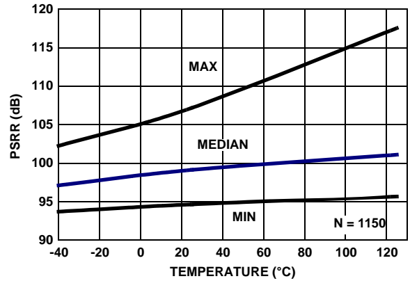
FIGURE 33. PSRR vs TEMPERATURE, V_+, V_- = \pm 1.2V \text{ TO } \pm 2.75V
