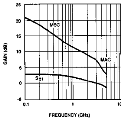
Figure 1. AT-60111 Insertion Power Gain, Maximum Available Gain, and Maximum Stable Gain vs. Frequency, V_{CE} = 3\text{ V} , I_C = 0.4\text{ mA} .
