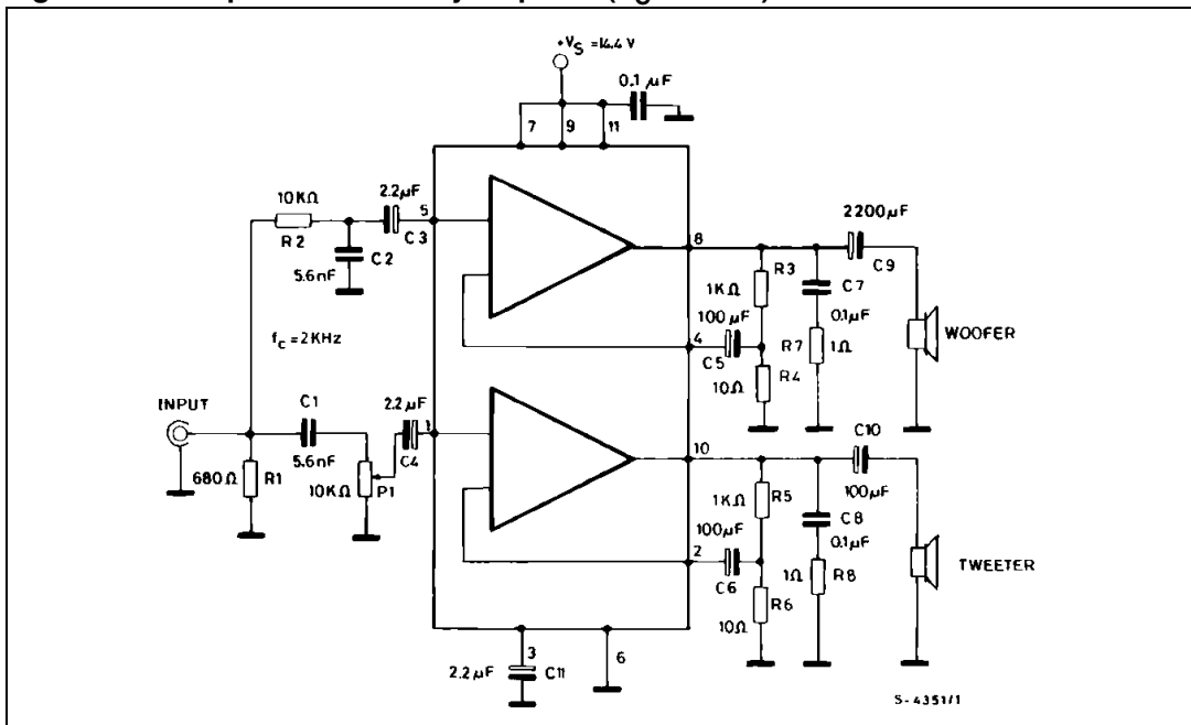
Figure 32. Simple 20 W two way amplifier ( F_C = 2 \text{ kHz} )
