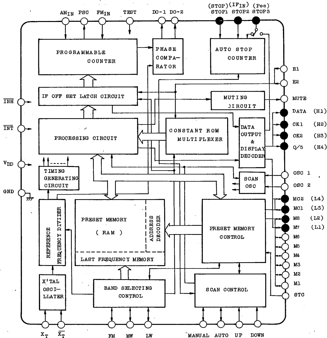
BLOCK DIAGRAM
