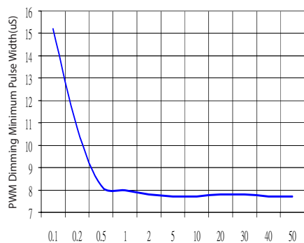
Condition: VIN = 12V, VOUT = 34.5V / 10mA x 4 strings
