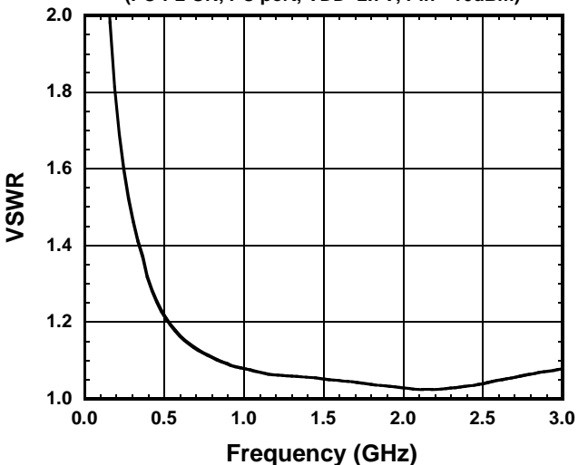
PC-P2 VSWR vs. Frequency
