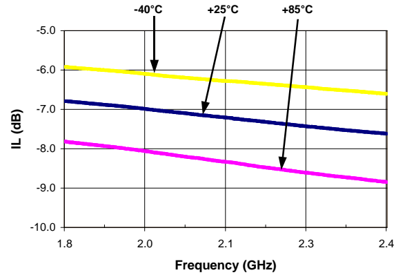
Insertion Loss vs. Frequency over Temperature at 750 pS State
