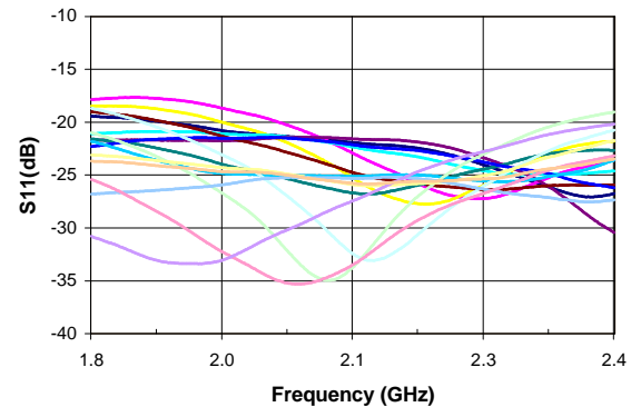
Output Return Loss vs. Frequency (+85°C)
