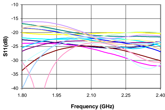
Input Return Loss vs. Frequency (+85°C)
