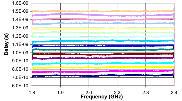
Delay vs. Frequency
