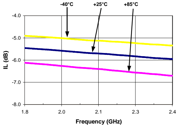
Insertion Loss vs. Frequency over Temperature at 0 pS State
