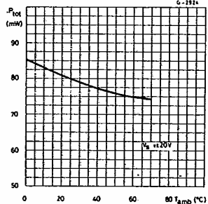
Fig. 26 - Power consumption vs. ambient temperature
