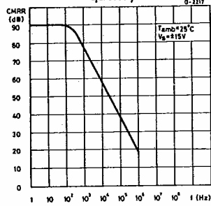
Fig. 14 - Common mode rejection ratio vs. frequency
