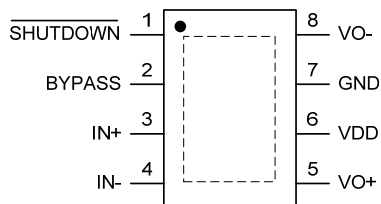
SOP8-PP Package (Top View)
