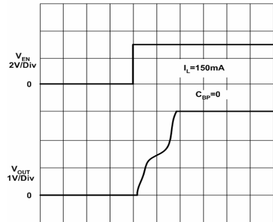
Enable Response ( V_{IN}=V_{OUT}+0.2V )
