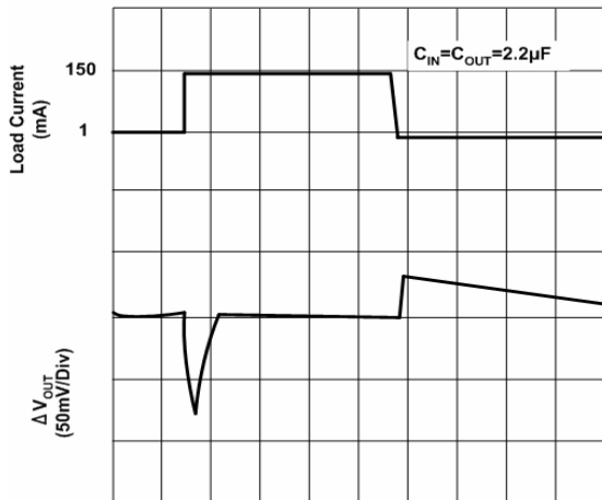
Load Transient Response ( V_{IN}=4.2V )
