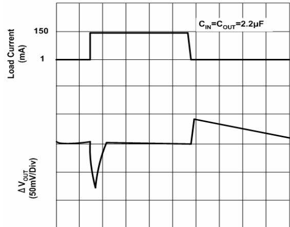
Load Transient Response ( V_{IN}=3.2V )
