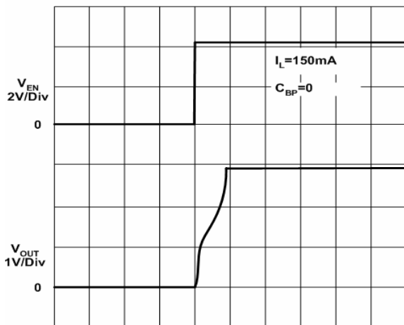
Enable Response ( V_{IN}=4.2V )
