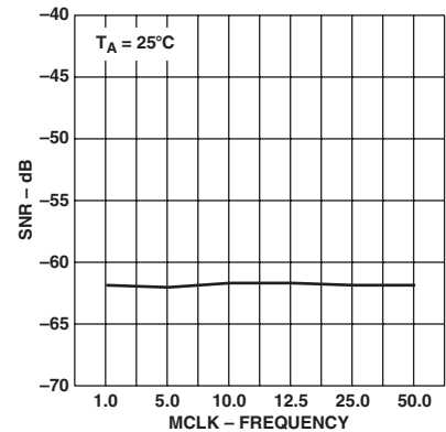
TPC 6. SNR vs. MCLK Frequency
