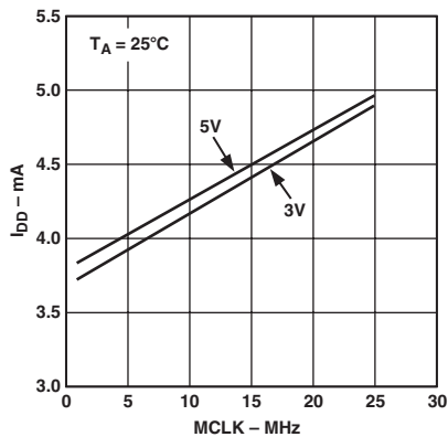
TPC 1. Typical Current Consumption vs. MCLK Frequency
