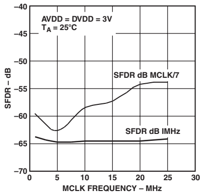
TPC 4. Wideband SFDR vs. MCLK Frequency
