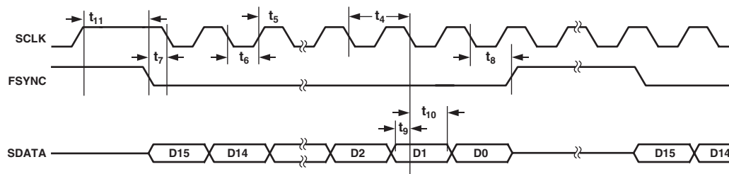
Figure 3. Serial Timing
