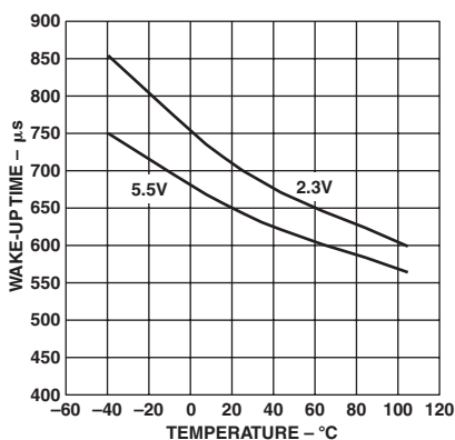
TPC 7. Wake-Up Time vs. Temperature
