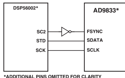
Figure 13. AD9833 to DSP56002 Interface
