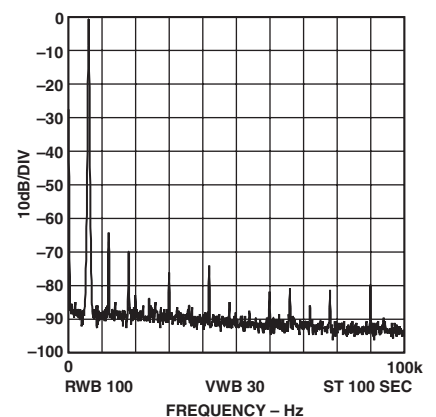
TPC 9. f_{MCLK} = 10 MHz, f_{OUT} = 2.4 kHz, Frequency Word = 000FBA9
