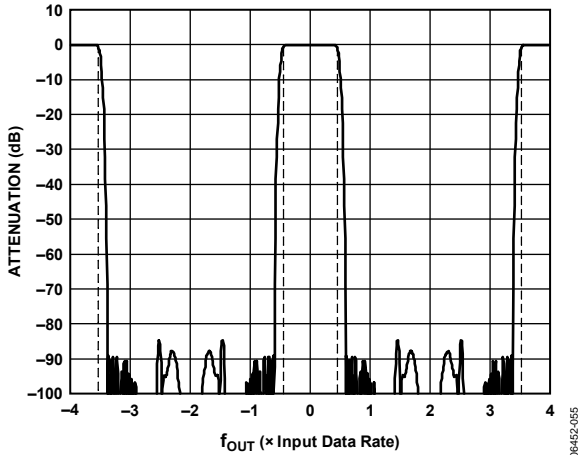
Figure 58. 4x Interpolation, Low-Pass Response to ±4x Input Data Rate (Dotted Lines Indicate 1 dB Roll-Off)
