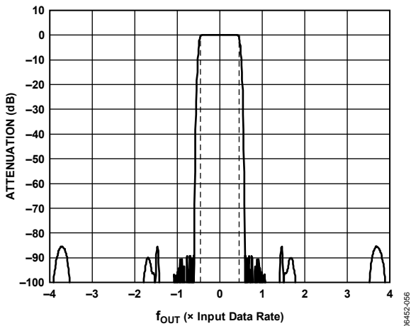
Figure 59. 8x Interpolation, Low-Pass Response to ±4x Input Data Rate (Dotted Lines Indicate 1 dB Roll-Off)
