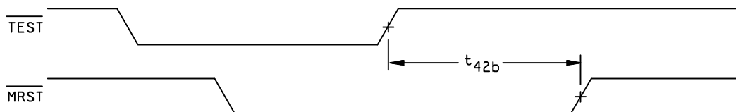
MASTER RESET TIMING WHEN TEST IS ACTIVE
