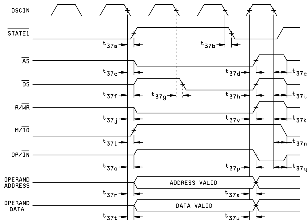
MEM WRITE CYCLE
