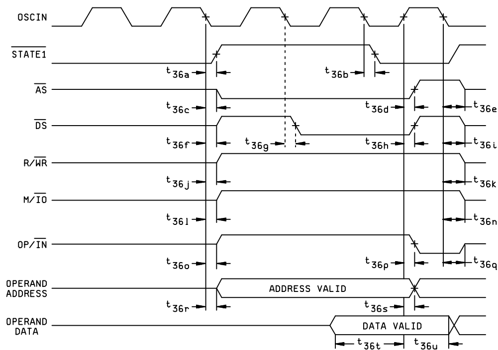
MEM READ CYCLE
