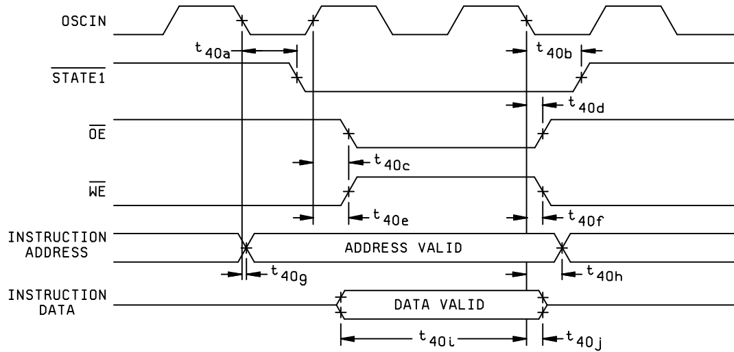
LRI COMMAND, RISC READ TIMING
