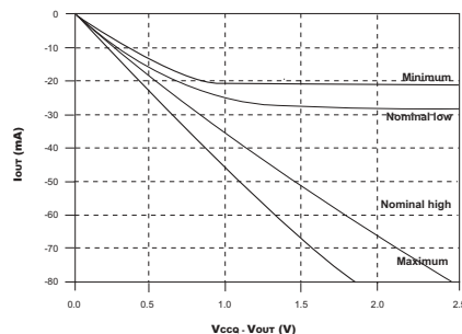
FIG. D PULL-UP CHARACTERISTICS
