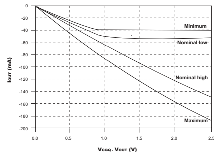
FIG. B PULL-UP CHARACTERISTICS
