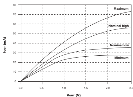
FIG. C PULL-DOWN CHARACTERISTICS
