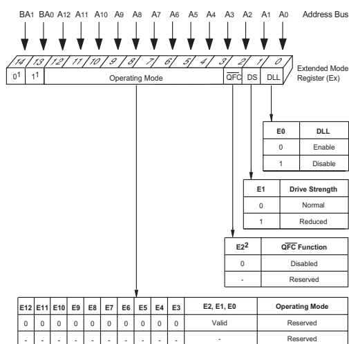
FIG. 5 EXTENDED MODE REGISTER DEFINITION
