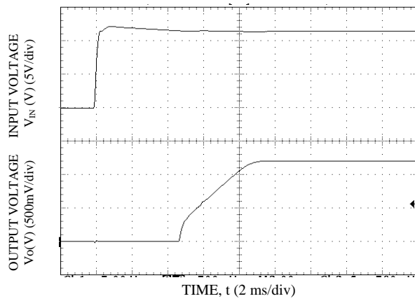
Start-up Using Input Voltage ( V_{IN} = 12V , I_o = I_{o,max} ), V_o = 1.2V , T_a = 25^\circ C
