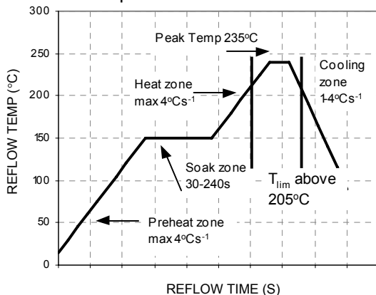
Reflow Profile for Tin/Lead (Sn/Pb) process
