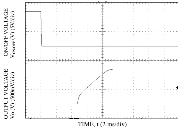
Start-up Using On/Off Voltage ( I_o = I_{o,max} ) V_o=1.2V , V_{in} = 12V , T_a=25^\circ C
