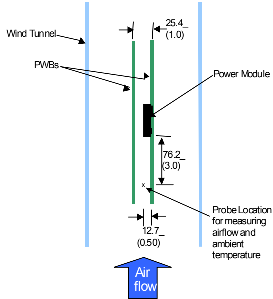
Thermal Test Setup
