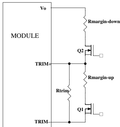
Circuit Configuration for margining Output voltage
