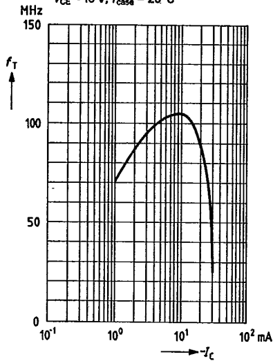
Transition frequency f_T = f(I_C) - V_{CE} = 10 V; T_{case} = 25^\circ C
