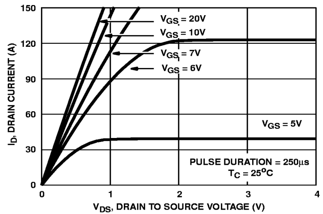
FIGURE 7. SATURATION CHARACTERISTICS
