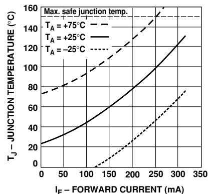
Figure 3. Junction Temperature vs. Forward Current as a Function of Heat Sink Temperature for the HSMS-2700 and HSMS-2702. Note: Data is calculated from SPICE parameters.
