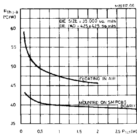
Figure 7 : PLCC68.
