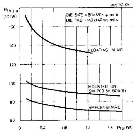
Figure 7 : PLCC68.
