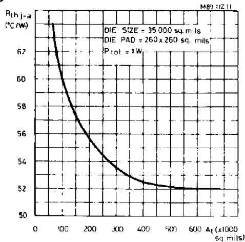
Figure 11 : PLCC44.
