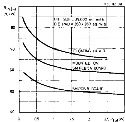
Figure 8 : PLCC84.
