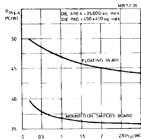
Figure 8 : PLCC84.
