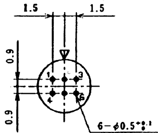
Size 7, 6 conductors
