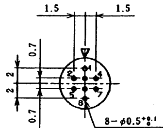
Size 7, 8 conductors
