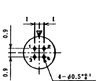
Size 7, 4 conductors
