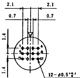
Size 9, 12 conductors
