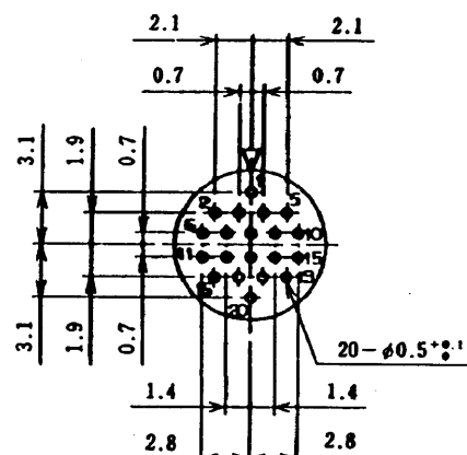
Size 9, 20 conductors
