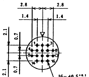
Size 9, 16 conductors
