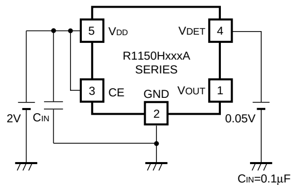
VDET Output Current Test Circuit
