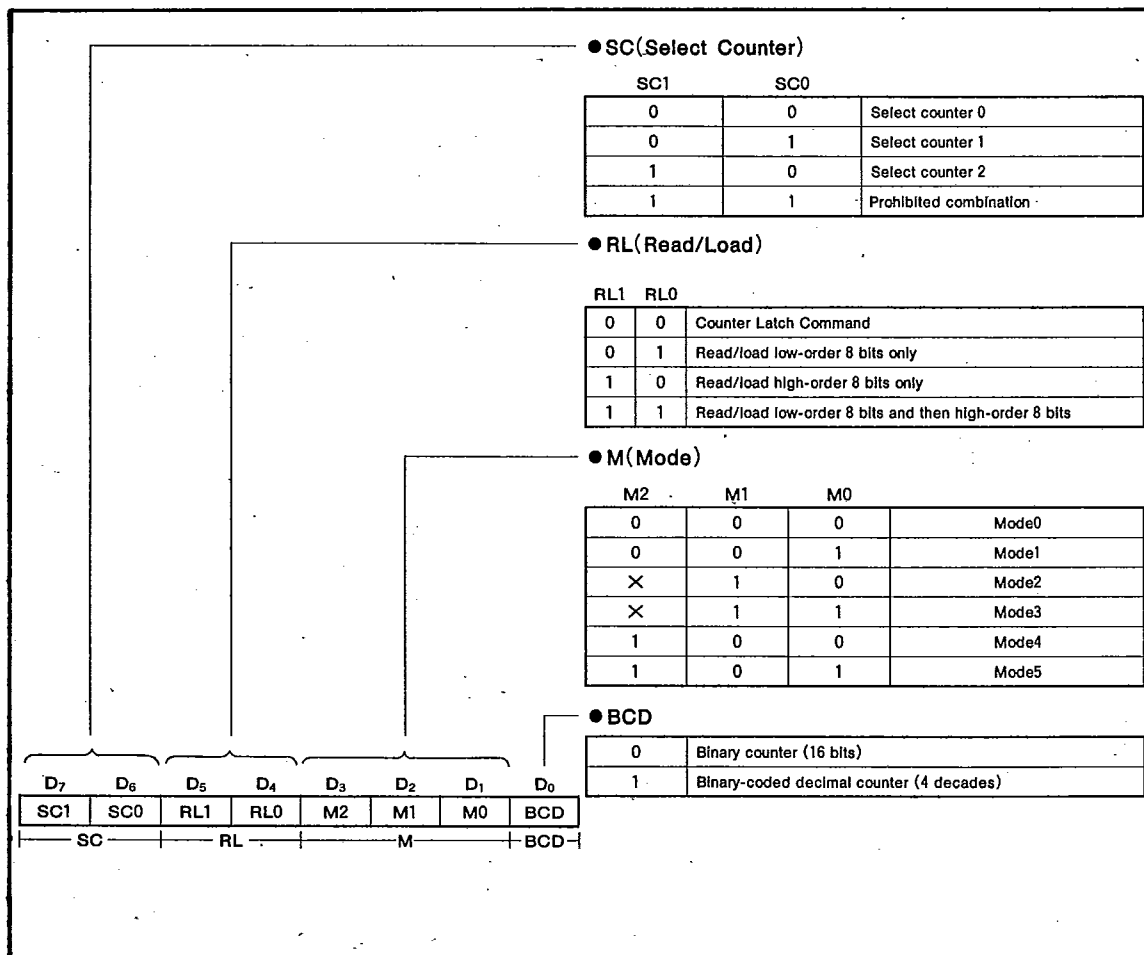
Fig. 1 Control-Word Format
