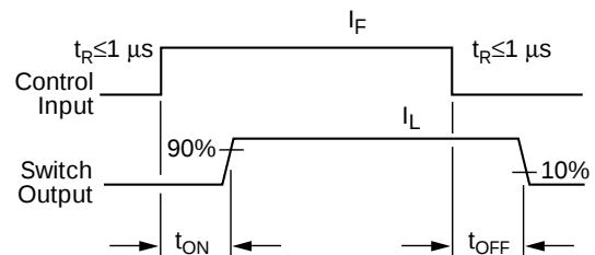
Figure 14. Switching waveform
