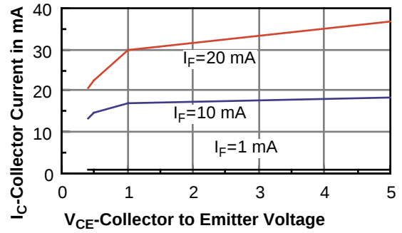
Figure 9. Collector current vs. collector voltage
