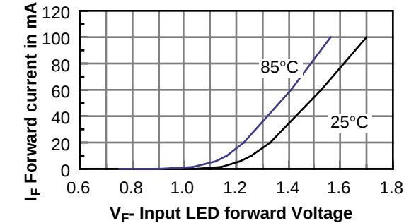
Figure 2. LED forward current vs. forward voltage
