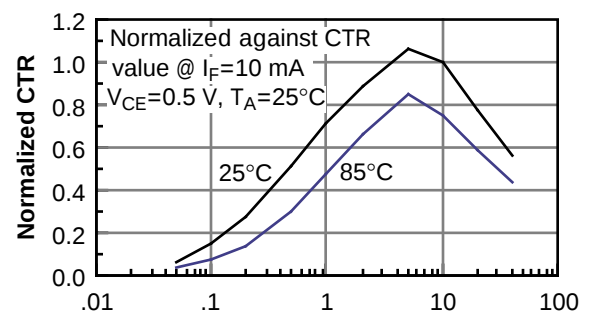
Figure 12. Non-saturated current transfer ratio
