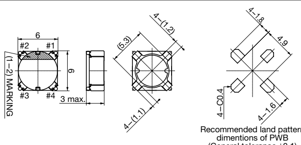
Recommended land pattern dimensions of PWB (General tolerance \pm 0.1 )
