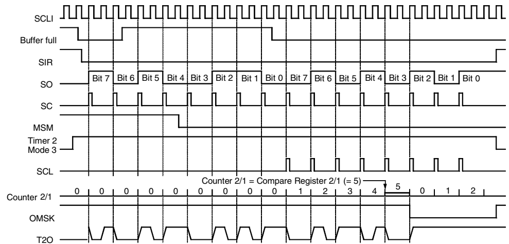
Figure 57. Bi-phase Modulation 2
