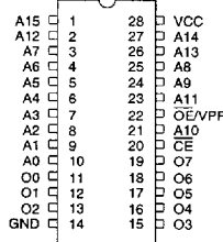
CDIP, PDIP, SOIC Top
