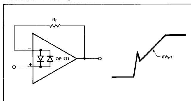
FIGURE 9: Pulsed Operation
