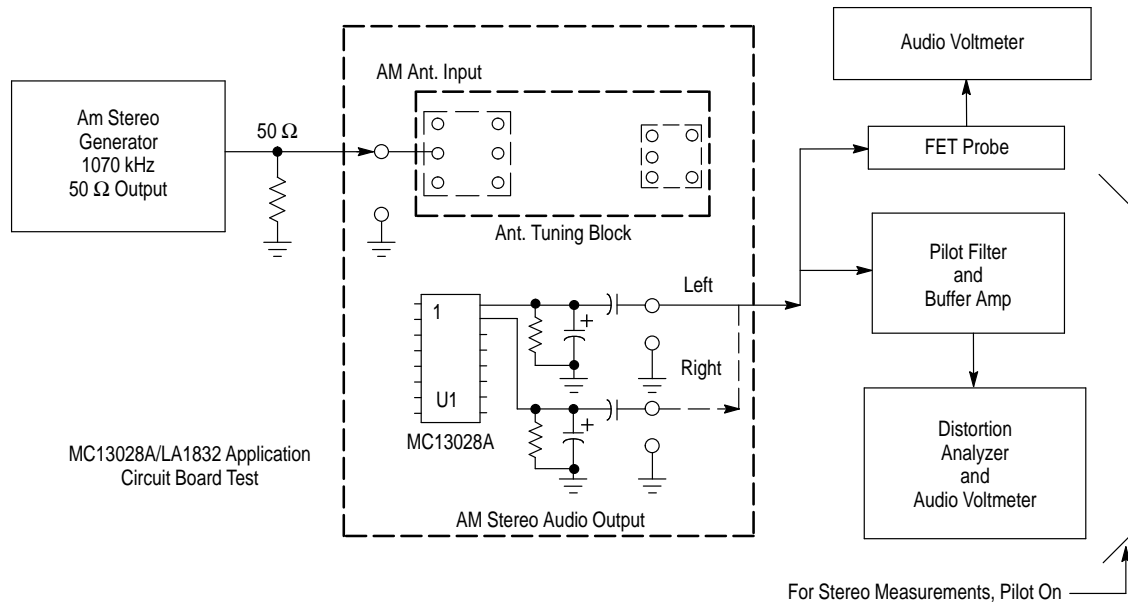
Figure 22. MC13028A/LA1832 Application Circuit Board Test Setup
