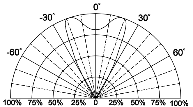
Fig.6 Directivity Radiation
