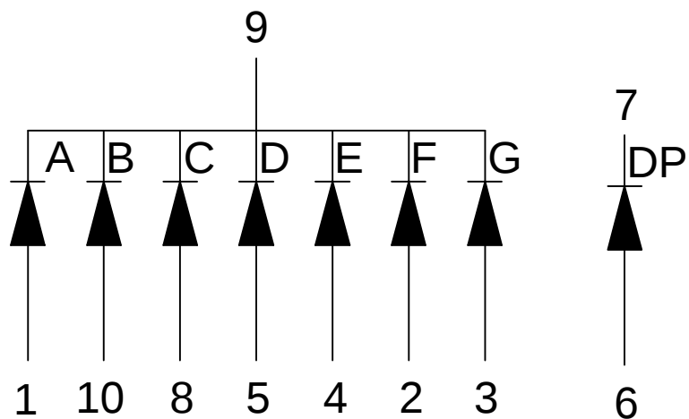
LSD3C55-XX-PF
