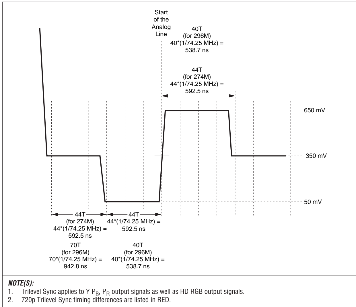
www.DataSheet4U.com Figure E-3. 1080i and 720p Trilevel Sync provided by CX25870/871
