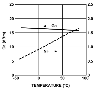
Figure 14. AT-30511 Noise Figure and Associated Gain at V_{CE} = 2.7 V, I_C = 1 mA vs. Temperature in Test Circuit, Figure 1. (Circuit Losses De-embedded)
