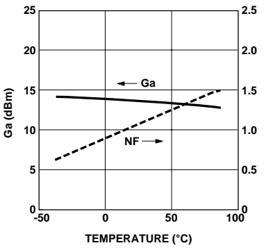
Figure 15. AT-30533 Noise Figure and Associated Gain at V_{CE} = 2.7 V, I_C = 1 mA vs. Temperature in Test Circuit, Figure 1. (Circuit Losses De-embedded)
