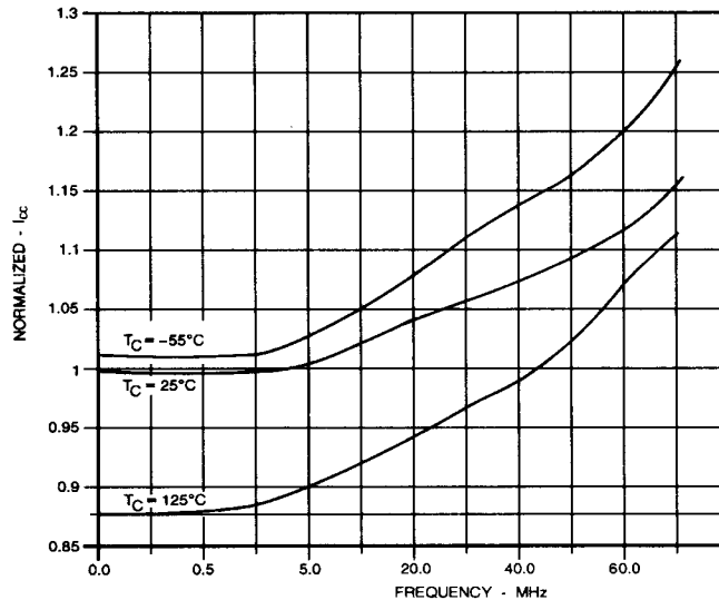
Figure 14. Am2925A I_{CC} Normalized vs Frequency ( V_{CC} = 5.5 \text{ V} )
