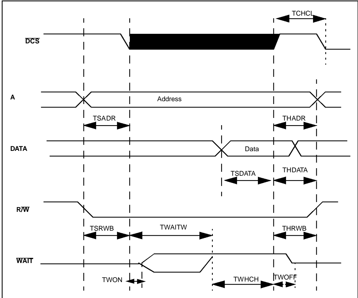
Figure 12. Write Access
