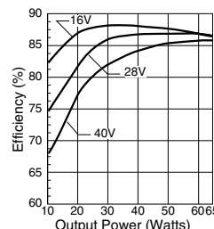
SMFL2815S & SMFL2815D Efficiency
