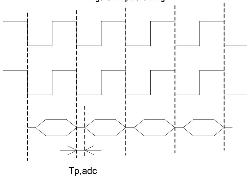
Figure 21. pixel timing
