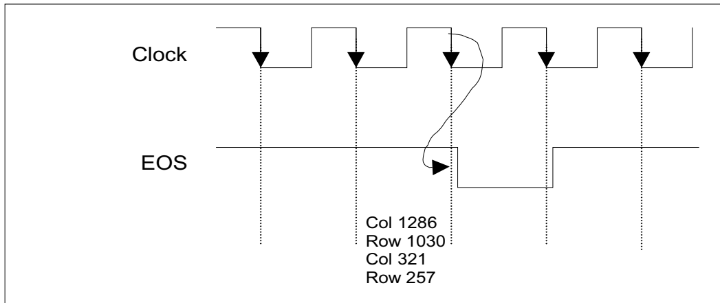
Figure 17. End-of-scan pulse
