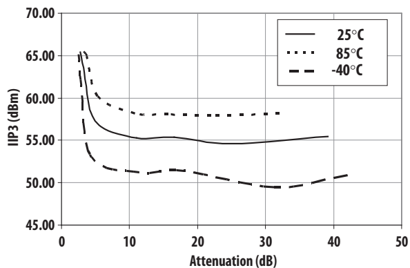
Figure 15. Input IP3 vs Attenuation vs Temperature at 900MHZ
