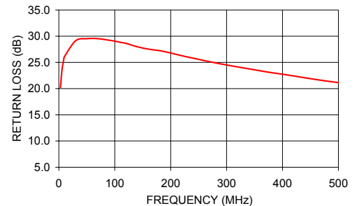
TC1.33-1T-75+ INPUT RETURN LOSS
