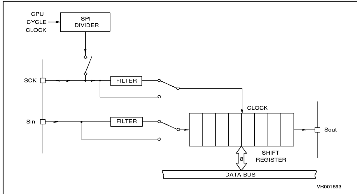
Figure 26. SPI Block Diagram
