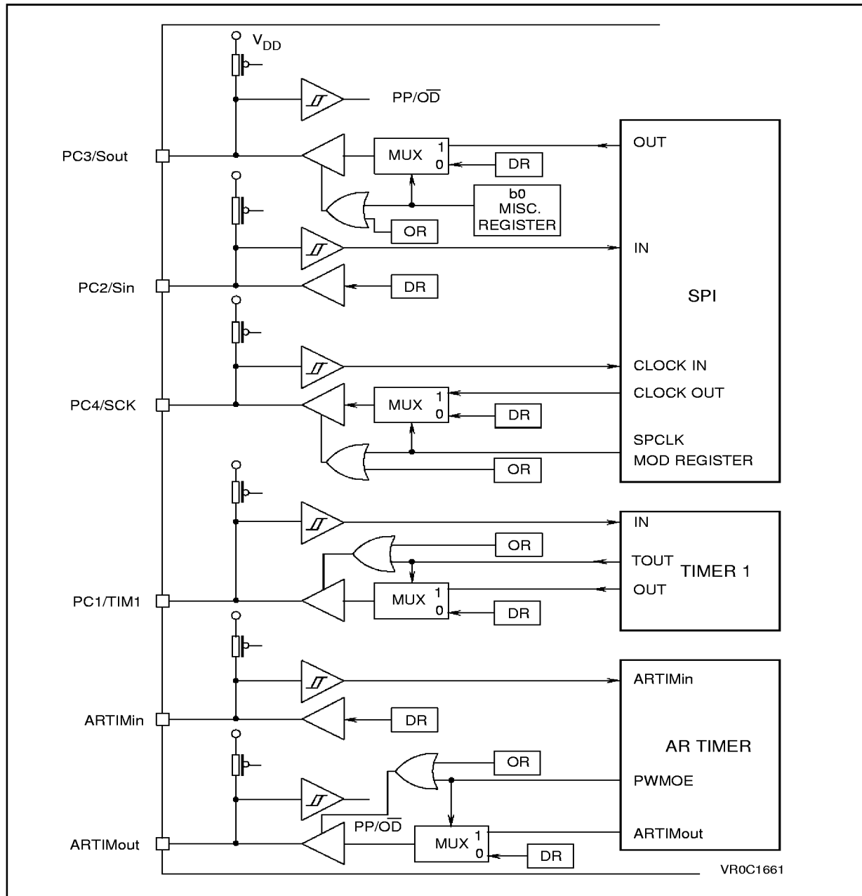
Figure 20. Peripheral Interface Configuration of SPI, Timer 1 and AR Timer
