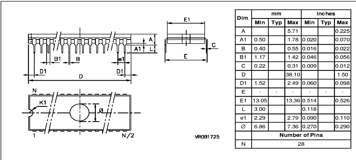
Figure 34. 28-Ceramic Dual In Line Package, 600-mil Width
