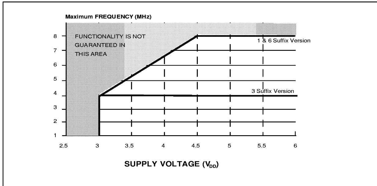
Figure 31. Maximum Operating FREQUENCY (Fmax) Versus SUPPLY VOLTAGE ( V_{DD} )
