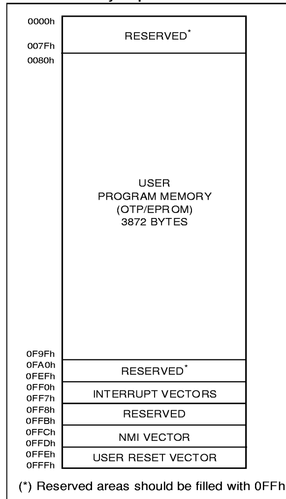
Figure 4. ST62T55B/T65B/E65B Program Memory Map
