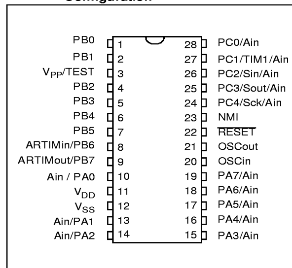
Figure 2. ST62T55B, T65B, E65B Pin Configuration
