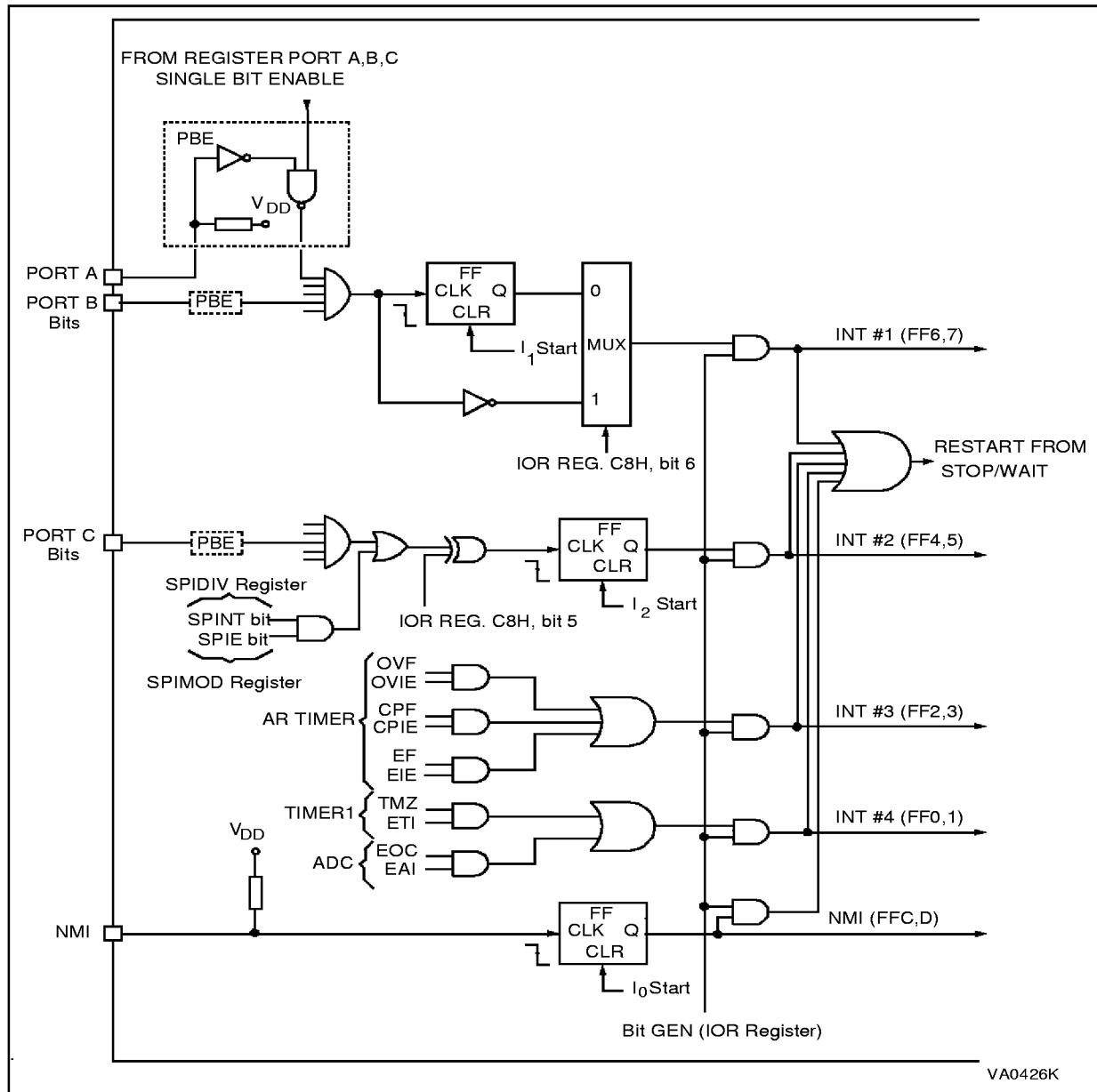
Figure 17. Interrupt Block Diagram
