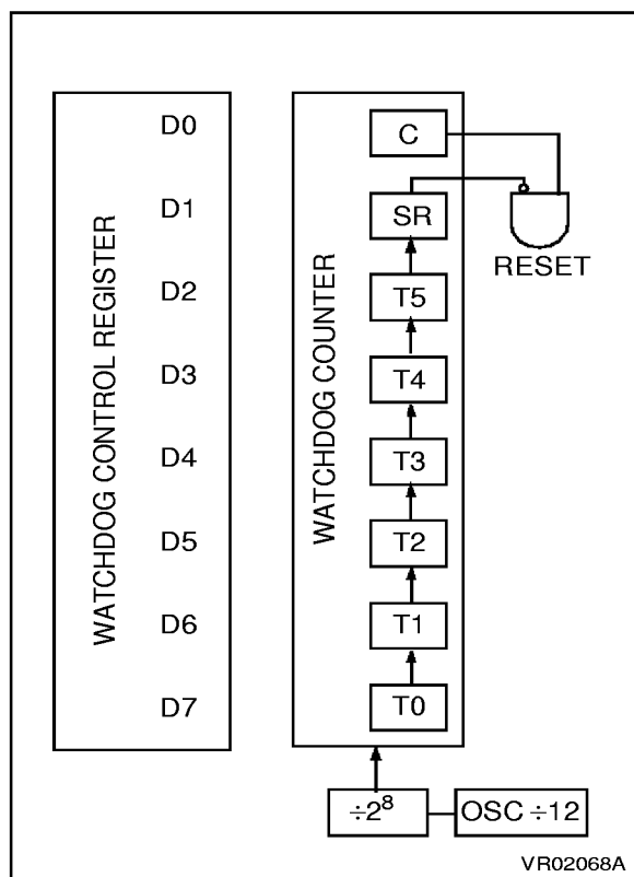
Figure 13. Watchdog Counter Control
