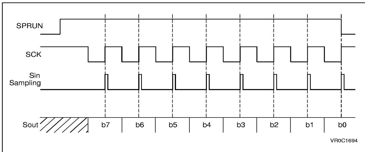
Figure 30. CPOL = 1 Clock Polarity Inverted, CPHA = 1 Phase Selection Shifted
