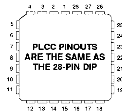
28-Pin PLCC
