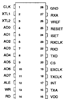
600-Mil 28-Pin DIP
