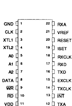
400-Mil 22-Pin DIP
