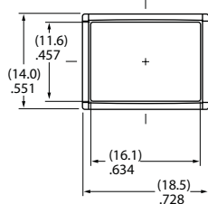
Rectangular • Barrier • Bushing Mount
