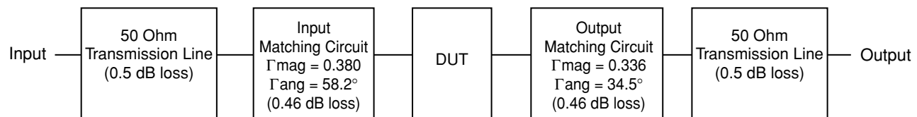
Figure 5. Block diagram of 2 GHz production test board used for Noise Figure, Associated Gain, P_{1\text{dB}} , and OIP3 measurements. This circuit represents a trade-off between an optimal noise match and a realizable match based on production test board requirements. Circuit losses have been de-embedded from actual measurements.
