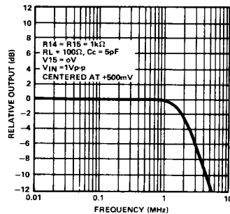
REFERENCE AMPLIFIER LARGE-SIGNAL FREQUENCY RESPONSE
