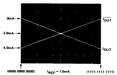
TRUE AND COMPLEMENTARY OUTPUT OPERATION
