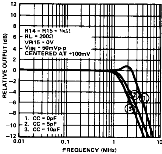
REFERENCE AMPLIFIER SMALL-SIGNAL FREQUENCY RESPONSE
