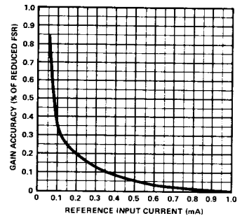
GAIN ACCURACY vs REFERENCE CURRENT
