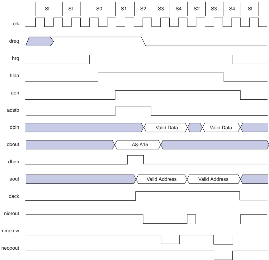
Figure 3. a8237 Timing Waveforms (Part 1 of 3)
