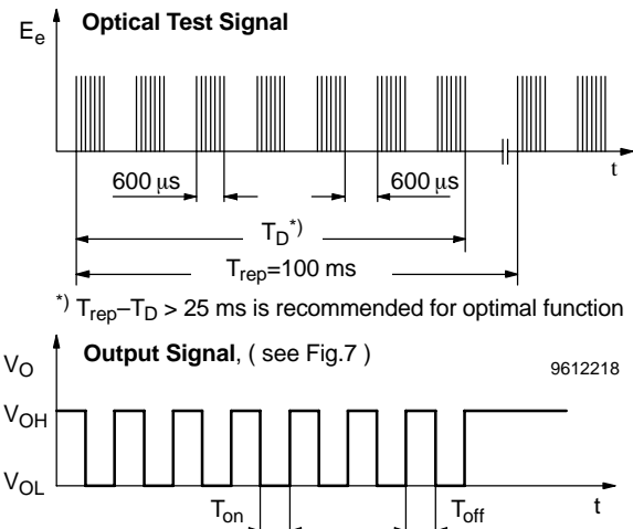
Figure 6. Output Function
