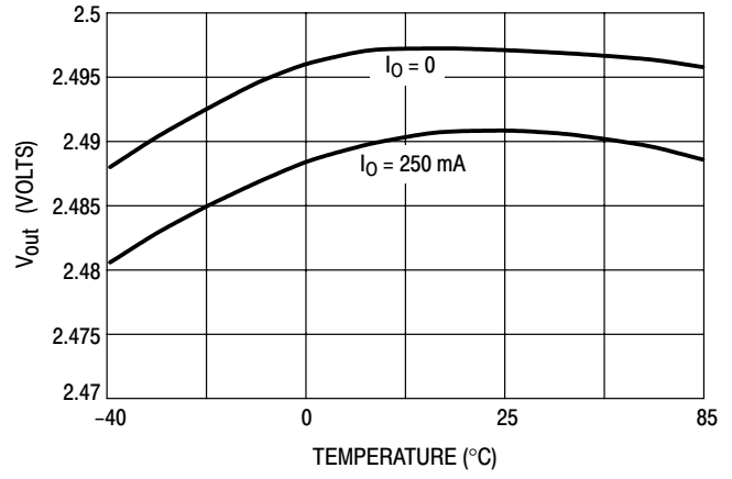
Figure 10. Output Voltage versus Ambient Temperature ( V_{in} = V_{out1} + 1V )
