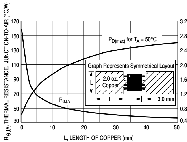
Figure 18. SOP-8 Thermal Resistance and Maximum Power Dissipation versus P.C.B. Copper Length
