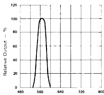
Wavelength (λ) — nm. Fig. 2 SPECTRAL RESPONSE.
