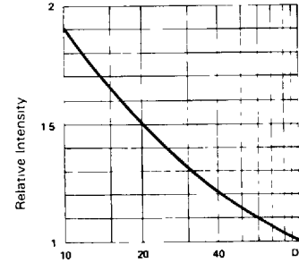
Fig 6 LUMINOUS INTENSITY Vs DUTY CYCLE% (AVERAGE I_a = 10\text{mA} PER SEG)
